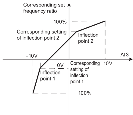
Fig 6-18 typical application case 3 of AI curve (4-points)
