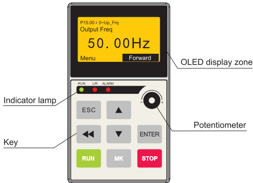
Fig 4-2 OLED keypad introduction
