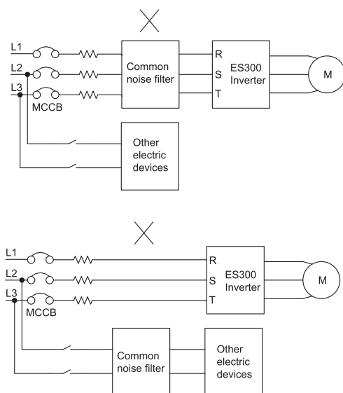
Fig 3-16 false wiring of noise filter
