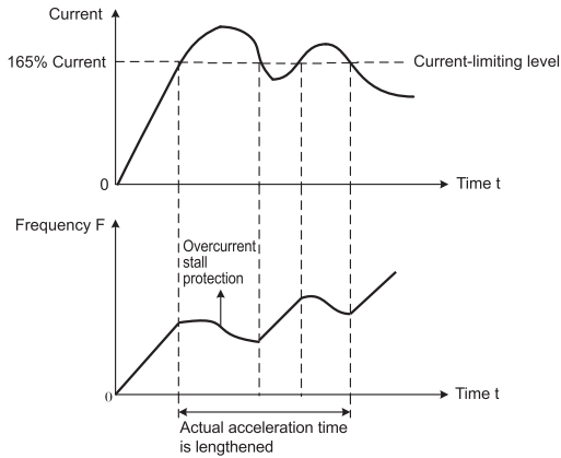
Fig 6-28 overcurrent stall protection
