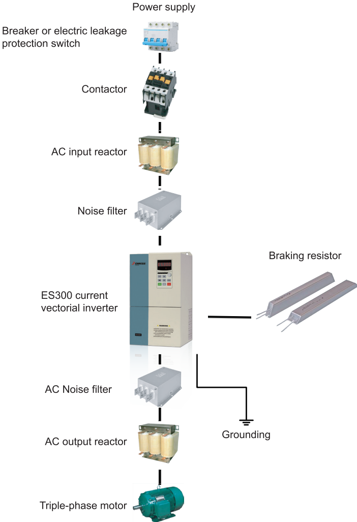
Fig 3-6 wiring diagram of inverter and peripheral equipment
