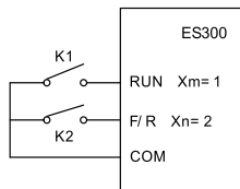
Fig 6-9: 2-thread control 1
