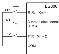
Fig 6-12 3-thread control 2
