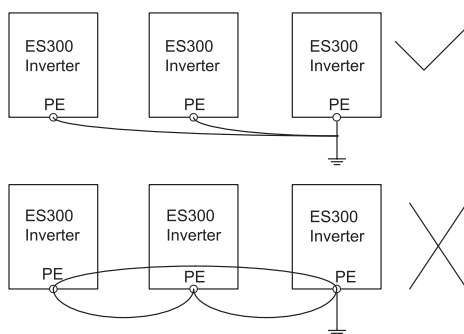
Fig 3-19 recommended grounding way
