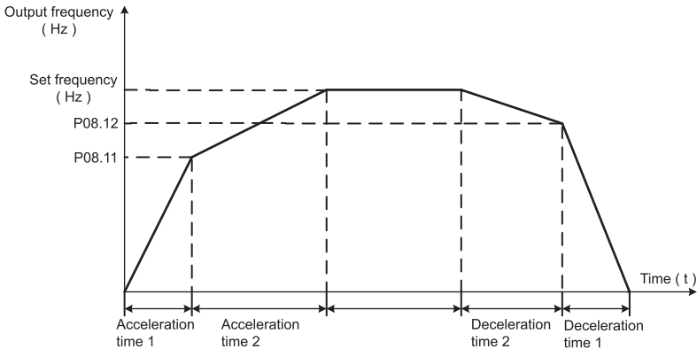
Fig 6-20 acceleration/deceleration time switching diagram
