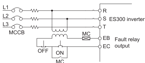
Fig 3-1 main circuit breaker wiring diagram
