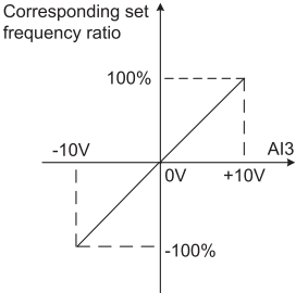
Fig 6-15 typical application 3 of AI curve (2-point) setting
