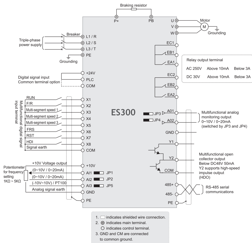
Fig 3-7 standard connection of main circuit and control circuit
