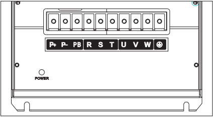
Fig 3-8 main circuit terminals diagram of ES300 18KW ~ 22KW ( Built-in braking unit )
