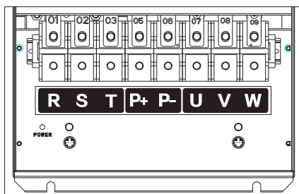
Fig 3-11 main circuit terminals diagram of ES300 75KW ~ 110KW
