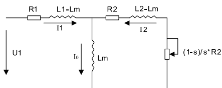
Fig 6-5 equivalent model of asynchronous motor in steady state
