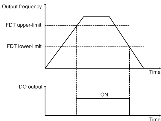
Fig 6-22 FDT frequency output level
