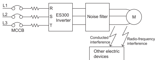
Fig 3-17 installation and wiring of noise filter on output side
