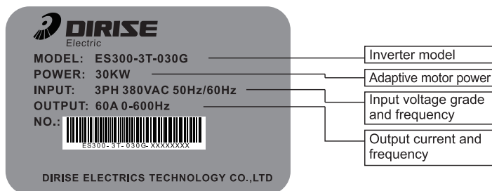
Fig 2-2 inverter nameplate
