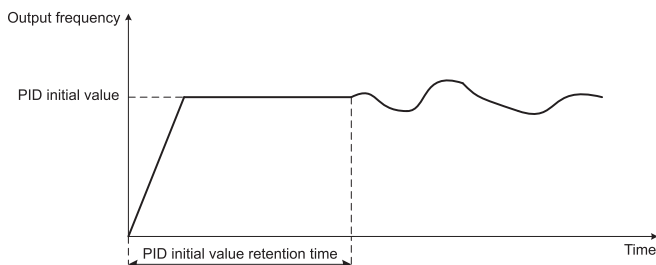
Fig 6-26 PID initial value retention time
