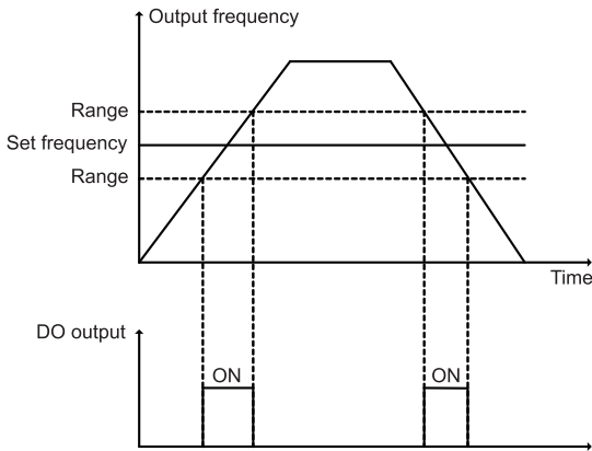
Fig 6-21 frequency arrival
