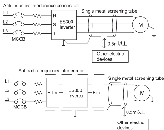
Fig 3-18 anti-interference installation wiring
