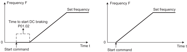
Fig 6-3 direct start diagram
