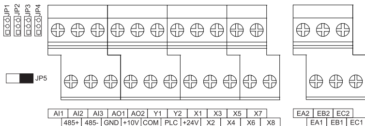
Fig 3-20 control circuit terminals
