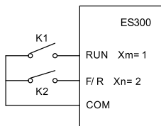
Fig 6-10: 2-thread control 2
