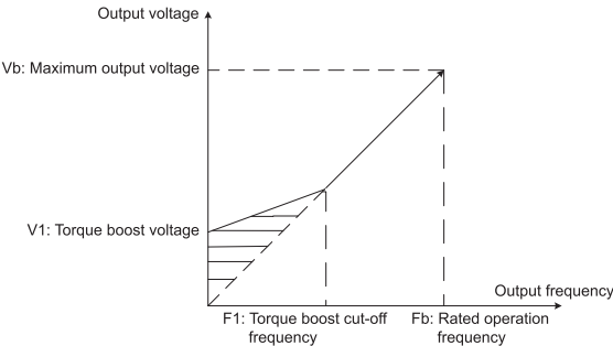
Fig 6-6 torque boost diagram
