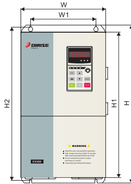
Fig 3-3 Fixation with bolts
