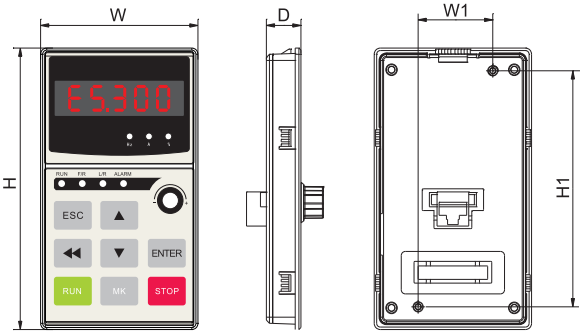
Fig 2-4 keypad installation dimension diagram (unit: mm)
