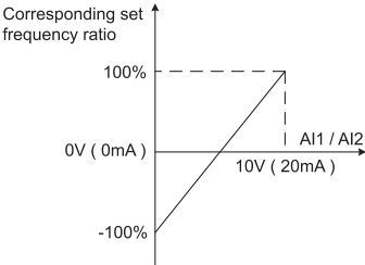
Fig 6-14 typical application 2 of AI curve (2-point) setting
