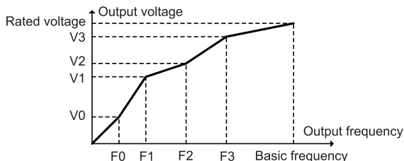
Fig 6-7 multi-points V/F curve diagram
