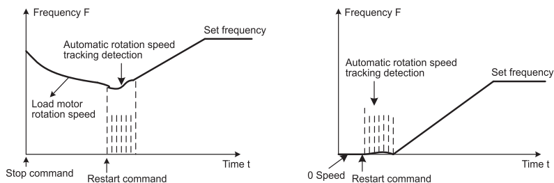
Fig 6-4 rotation speed tracking start diagram
