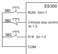
Fig 6-11: 3-thread control 1
