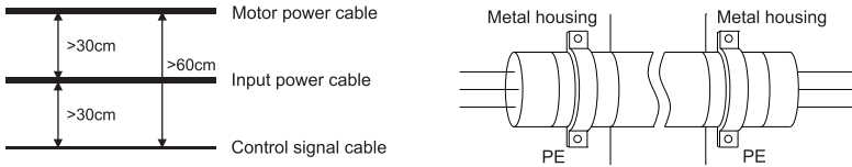
Fig 8-1 wiring requirement and shielded grounding way
