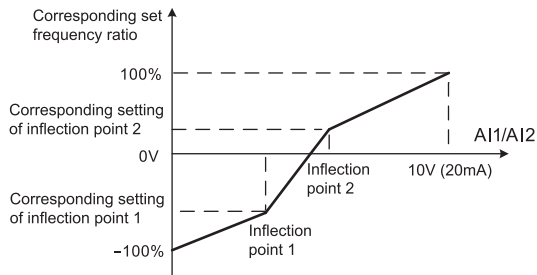
Fig 6-17 typical application case 2 of AI curve (4-points)
