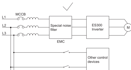
Fig 3-15 correct wiring of noise filter
