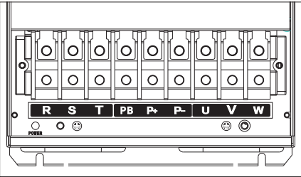
Fig 3-9 main circuit terminals diagram of ES300 30KW ~ 37KW ( Braking unit is selective )
