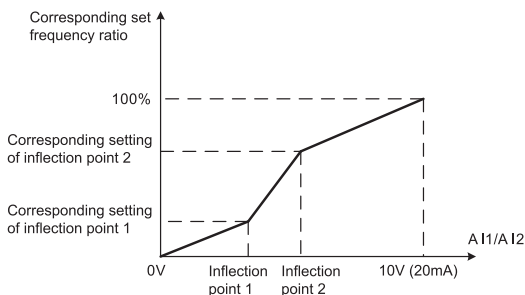
Fig 6-16 typical application case 1 of AI curve (4-points)
