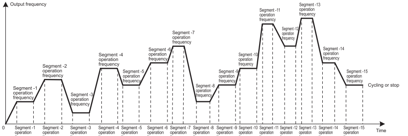
Fig 6-27 PLC multi-segment frequency operation
