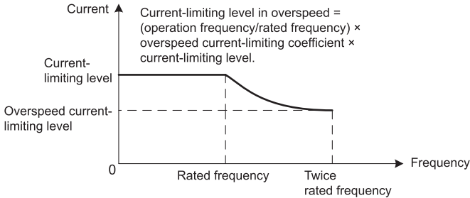
Fig 6-29 overspeed current-limiting level
