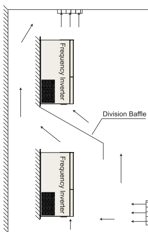
Fig 3-2 installation diagram of multiple inverters
