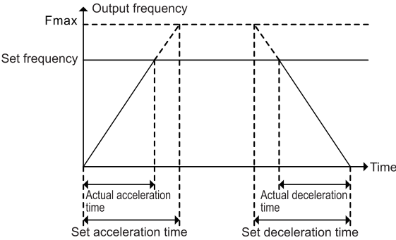
Fig 6-1 acceleration/deceleration time
