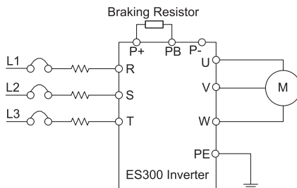
Fig 3-13 standard wiring diagram of main circuit
