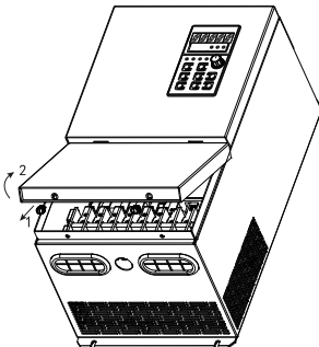
Fig 3-4 terminal cover disassembly
