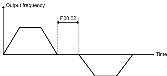
Fig 6-2 diagram of forward/reverse rotation dead-time
