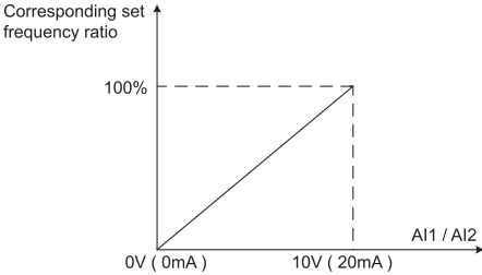
Fig 6-13 typical application 1 of AI curve (2-point) setting
