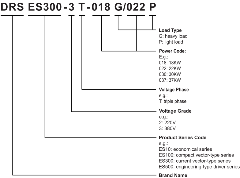
Fig 2-1 Model Description
