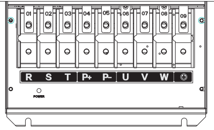
Fig 3-10 main circuit terminals diagram of ES300 45KW ~ 55KW
