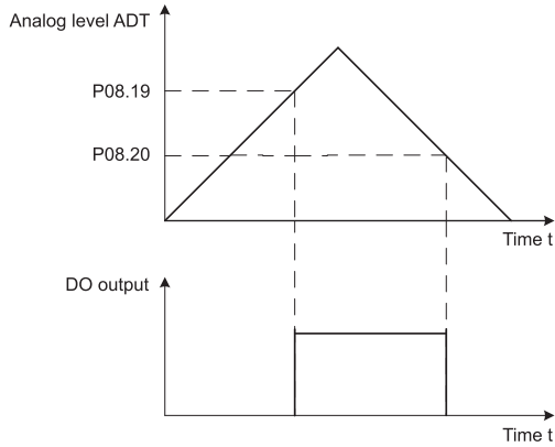
Fig 6-23 analog level ADT
