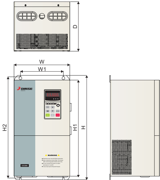
Fig 2-3 housing appearance and installation size of inverter 18.5KW ~ 400KW
