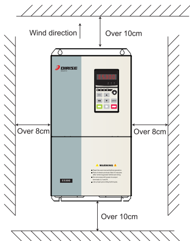
Fig 3-1 installation interval diagram
