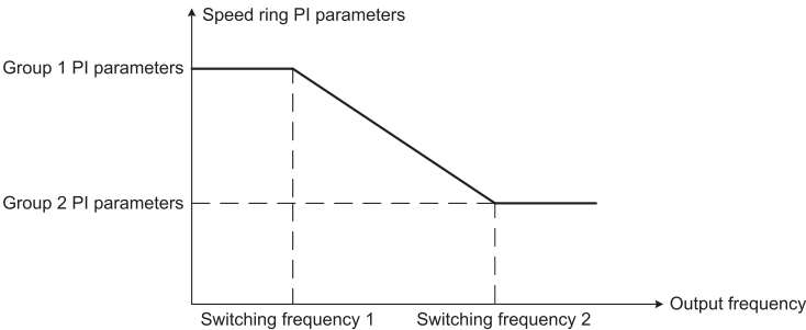
Fig 6-8 speed ring PI parameter switching diagram
