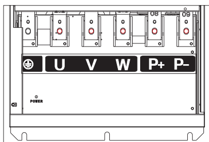
Fig 3-9 main circuit terminals diagram of ES300 132KW ~ 160KW
